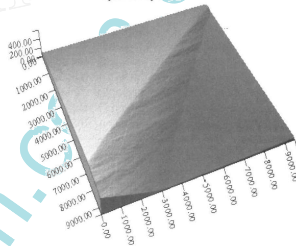
Figure 6. Diamond surface scan by AFM
