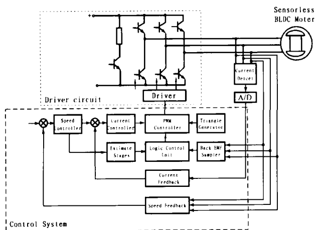
Figure 2. Closed-loop system of BLDC motor
