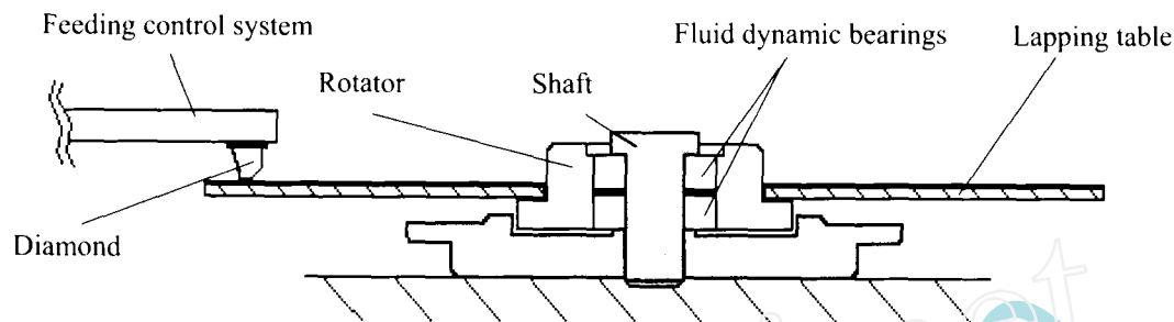
Figure 1 Diamond lapping system based on brushless DC motor spindle and fluid dynamic bearings
