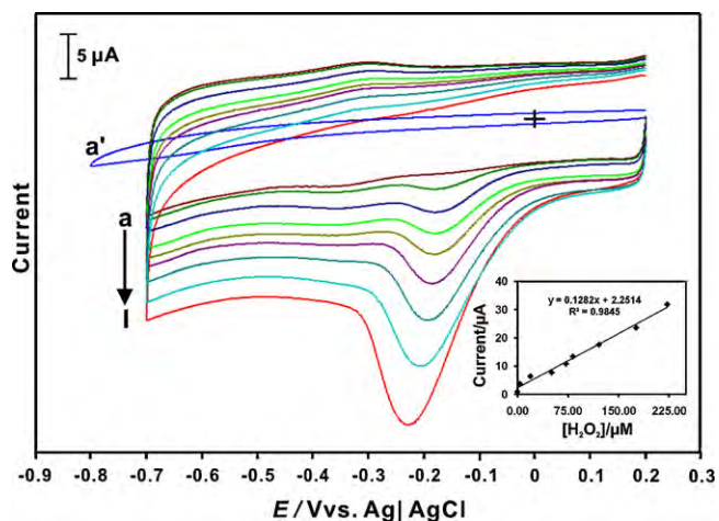
Fig. 9. Cyclic voltammograms obtained at NF/HRP/Bi 2 O 3 -MWCNT/GCE at the scan rate of 50 mV s -1 in the (a) absence and presence of (b) 3.6 (c) 19.2, (d) 50.9, (e) 72.0, (f) 82.2, (g) 121.0, (h) 176.0, and (i) 222.2 μM H 2 O 2 , (a') bare/GCE in the presence of 222.2 μM H 2 O 2 . Supporting electrolyte: N 2 saturated 0.05 M PBS (pH 7). Inset is the plot of cathodic peak current vs. [H 2 O 2 ].
